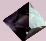
Fluorit in Oktaederform
